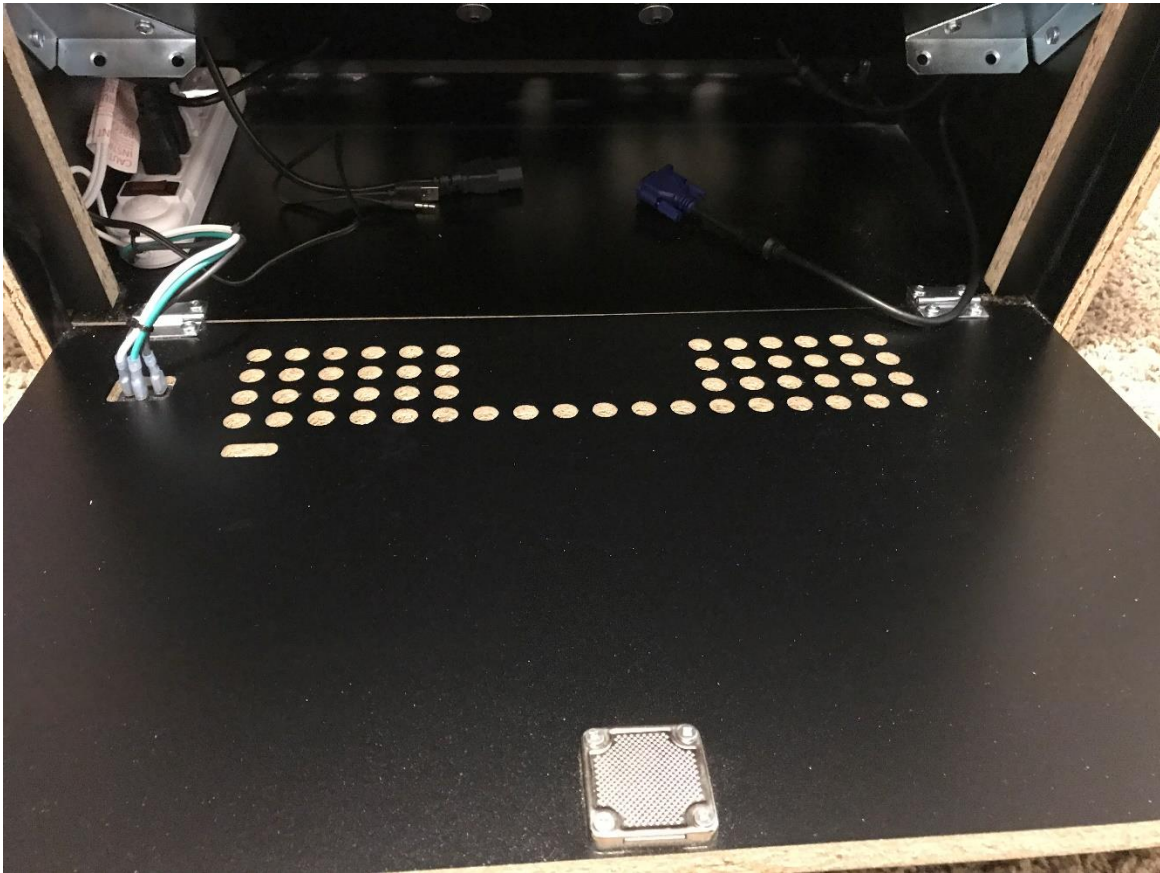
Below is an assembled cabinet with black L channel to hold Maquee plexiglass in place. I have installed a 22" LCD. Leave room for bezel and LCD plexiglass between speaker panel and LCD.
